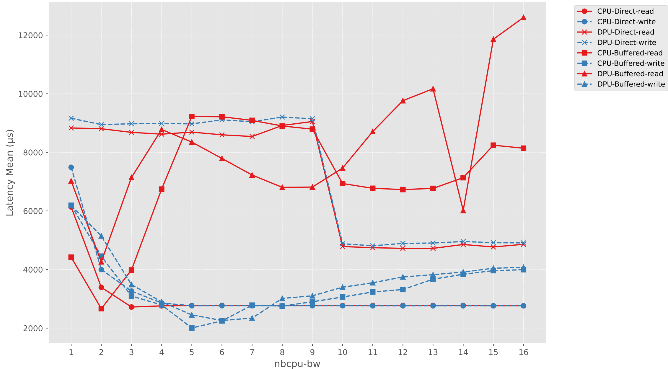
Latency Mean vs nbcpu-bw (CPU vs DPU, Direct vs Buffered)
